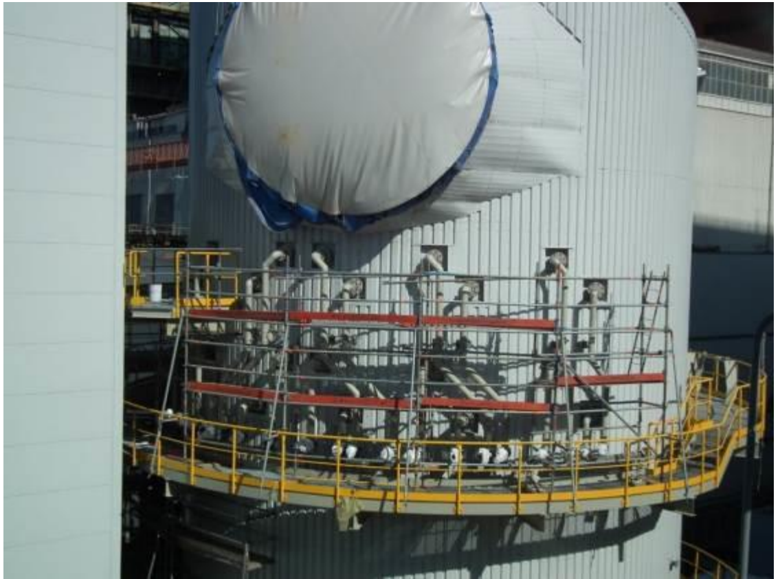
Equipment of the absorber and pump station building enabling the start-up of the desulphurisation technological line
